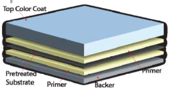
A two coat system with a Primer and Color Top Coat to pretreated substrate.
